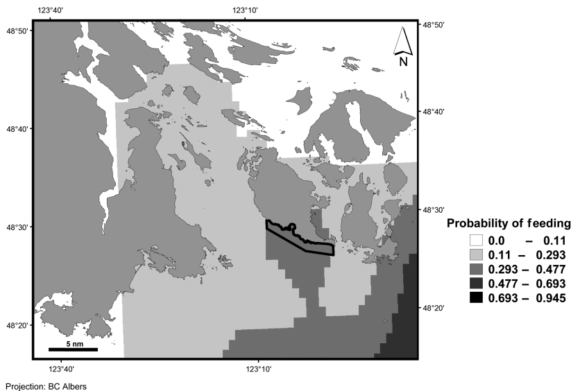
Figure 3 The predicted values of feeding throughout the study area (the greyscale values in each grid cell). The results from the classification tree identified the area between 48.4476°N and 48.4894°N as a high-probability area for feeding, so these limits are drawn as the northern and southern boundaries of our proposed marine protected area (MPA). Interviews with on-the-water environmental educators suggested that a 1 nautical mile area was considered manageable, so this defined the offshore boundary of our proposed MPA. Integrating all three sources of information, we identified a region up to 1 mile off south-western San Juan Island as a priority feeding area to propose for interim protection (dark outline).
